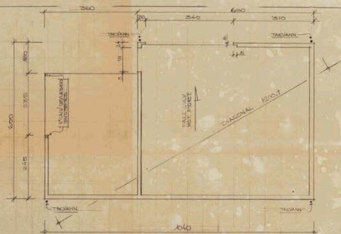
FUNDAMENTPLAN
