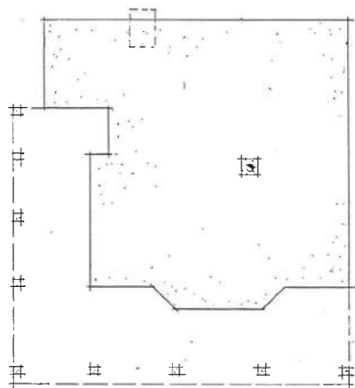
FUNDAMENTPLAN - M = 1:100
