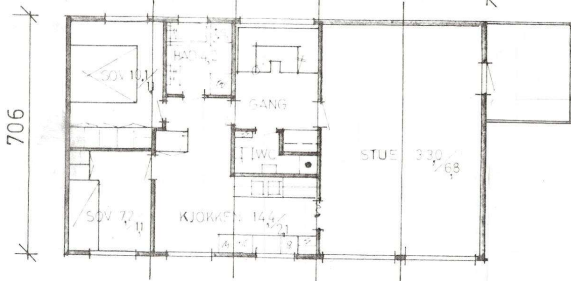
1 Etg plan
