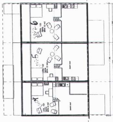
PLAN HEMS
