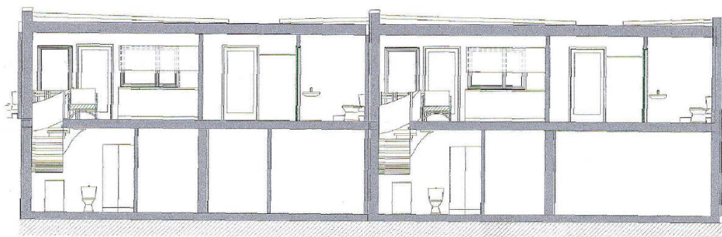
SNITT STUE / GANG / WC
