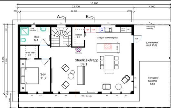
Plan 2
