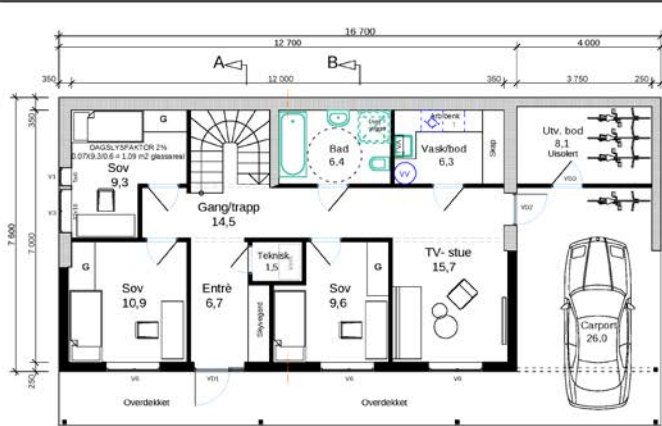
Plan 1
