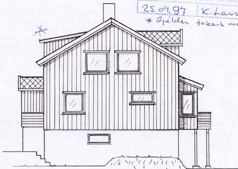
FASADE VEST.
