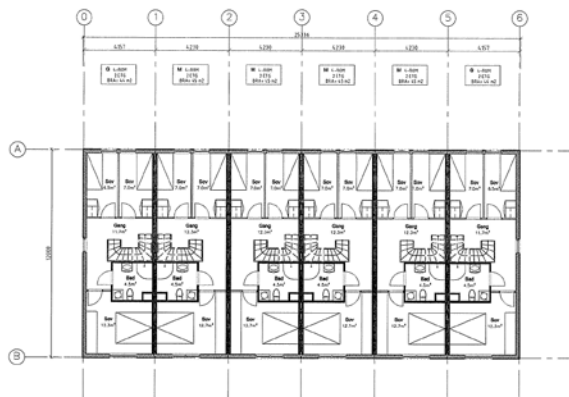
PLAN 2. etg. 1.888 m by 197.3 m
