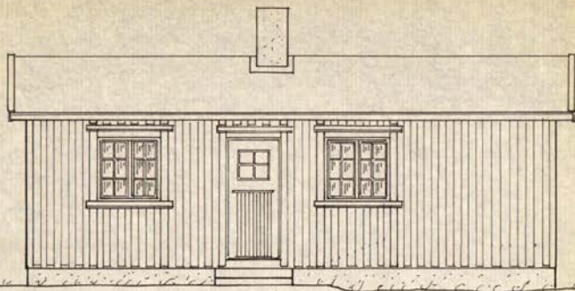
FASADE VEST.
