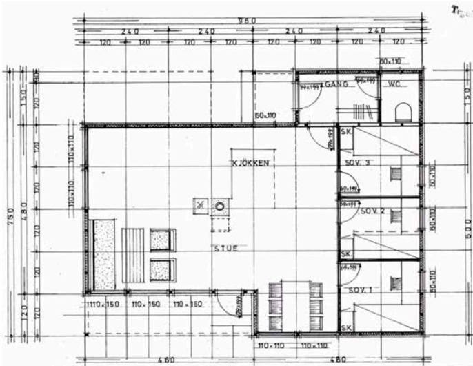
GRUNNRIS; (52+5) m 2 • M=1:50
