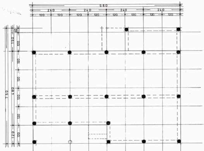
FUNDAMENTPLAN • M=1:50
