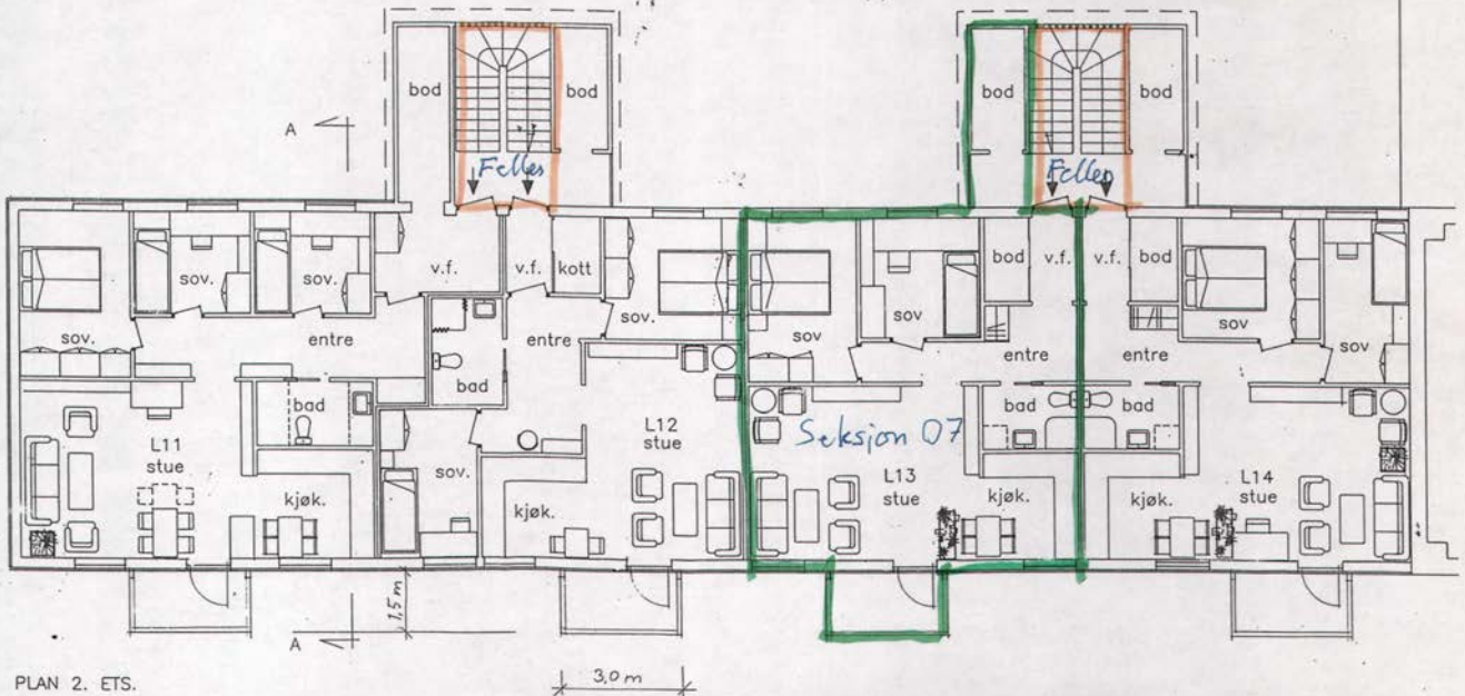
PLAN 2. ETS.
