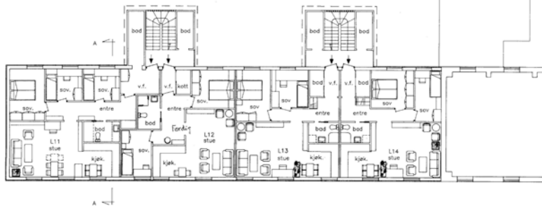
PLAN 2. ETS.
