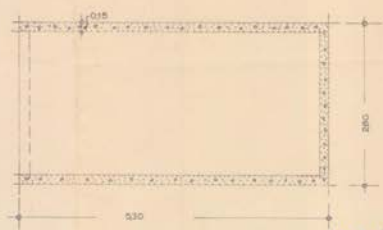
Fundamentplan
