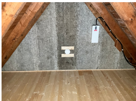
Ventiler for lufting.
