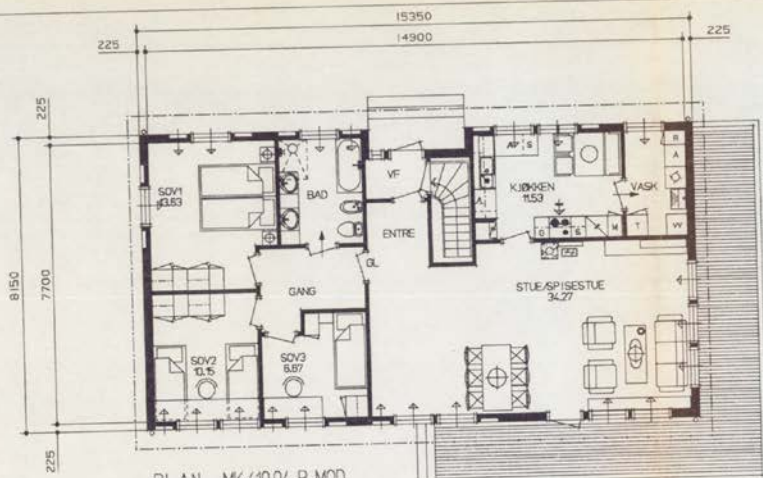
PLAN MK410.04-P-MOD
